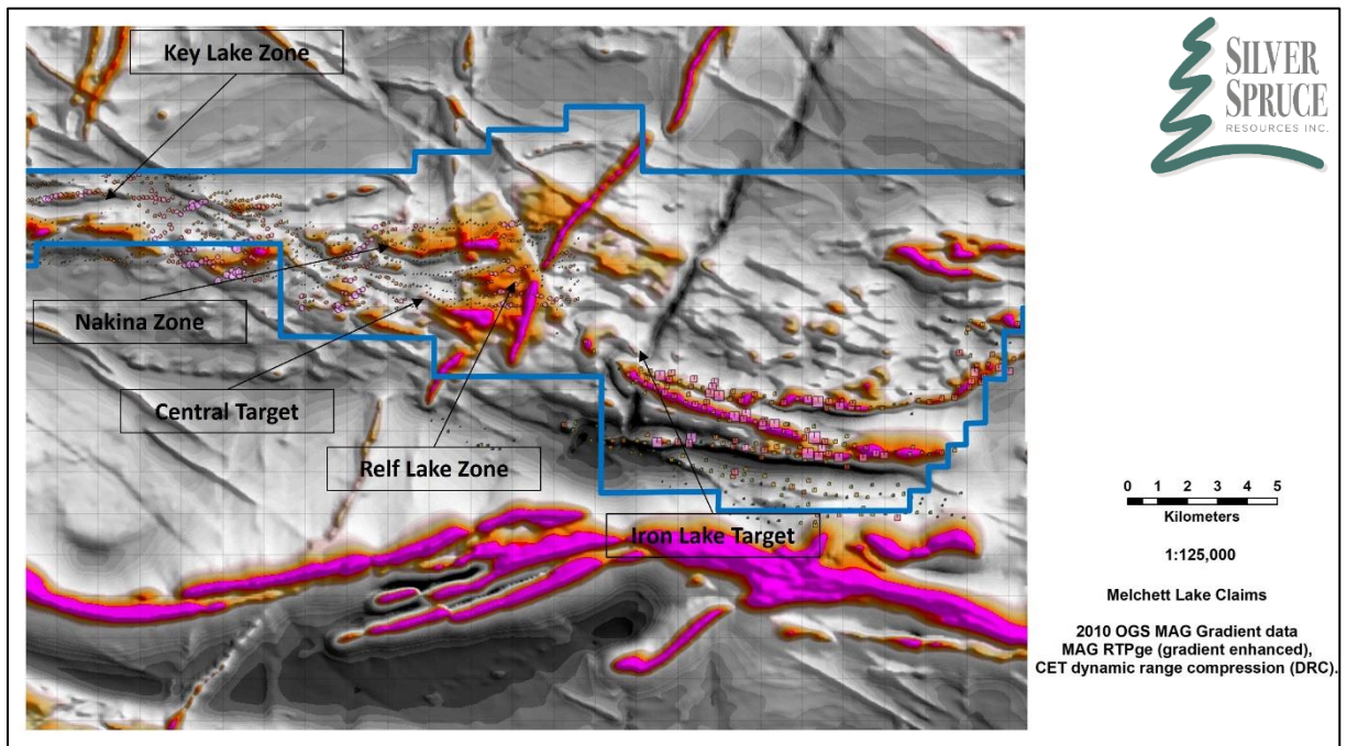
Figure 3. Melchett Lake claims (outlined in blue) showing magnetic gradient data and EM anomalies (pink squares with proportional size to strength), select NE and NW diabase dyke linears and tightly folded iron formation with high magnetic intensity (bright pink). Known zones of An-Ag-Cu-Au-Pb mineralization and target areas focused along coincident MAG/EM and structural loci.
