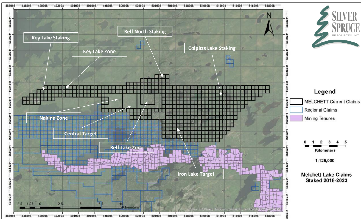
Figure 1. Melchett Lake claims (black cells) showing areas of recent staking by Company and Vendor (Key Lake and Relf North, and Colpitts Lake), known zones of An-Ag-Cu-Au-Pb mineralization, and additional targets with indicated geophysical, geochemical and/or geological anomalies.
